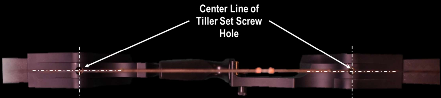
Figure 19 Limb Alignment Check
