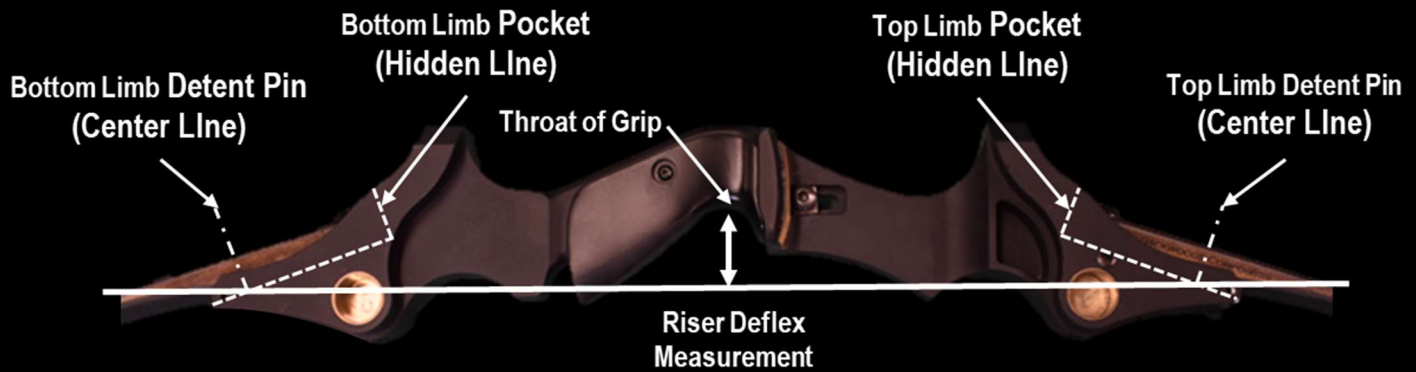
Figure 17 Riser Deflex Measurement
