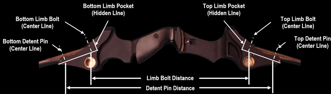
Figure 8 Limb Bolt Distance Measurement
