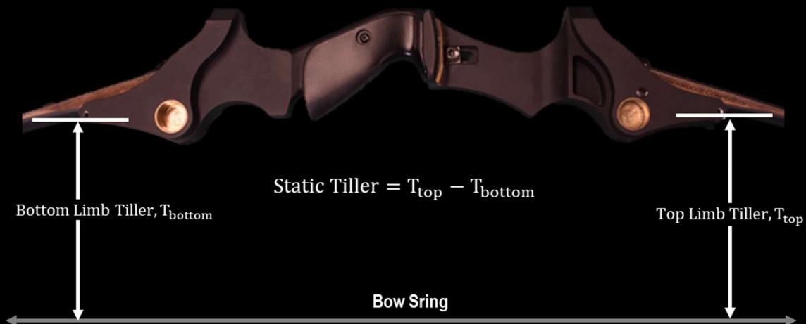
Figure 18 Tiller Measurement Locations
