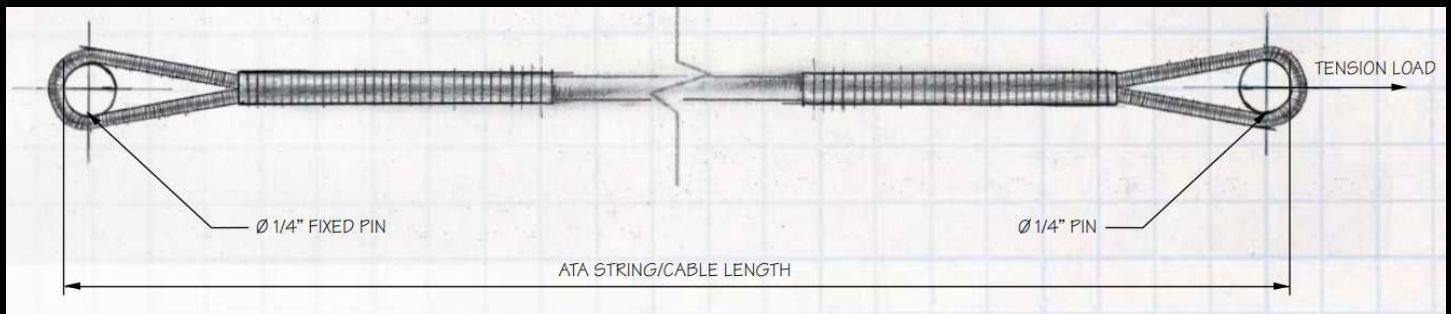
Figure 12 ATA String Length
